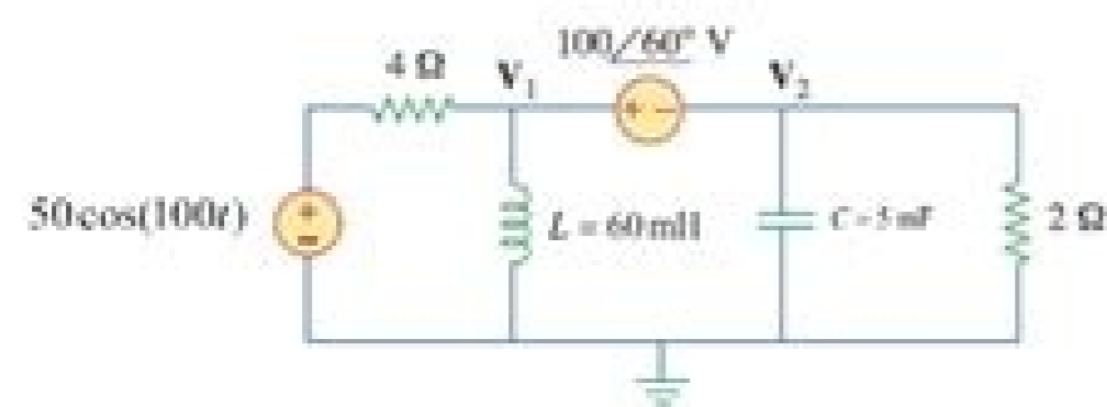
Fig. 3 Circuit for Question 3
